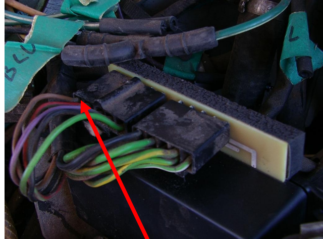
Pin 1 Brown wire
